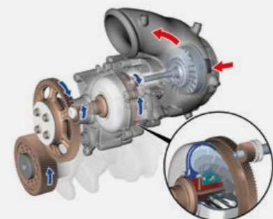
Turbo-compound technology for OM 473 LA
